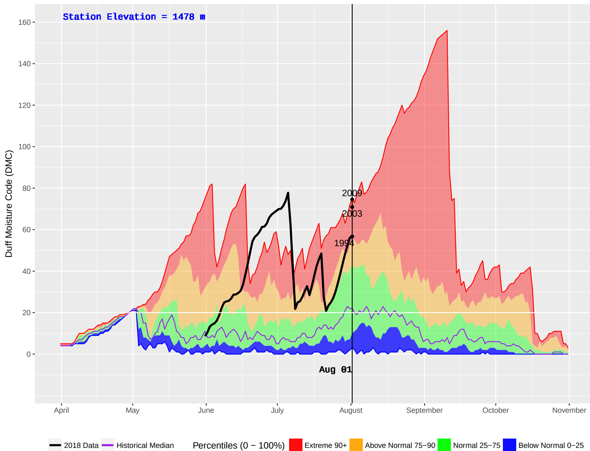
BERRY (267) : Historical (1989–2016) and Current (2018) Daily Duff Moisture Code (DMC)
